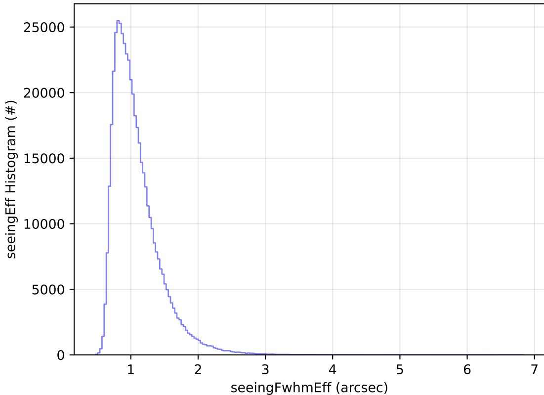
too_combined_no_nss_s10.0_v3.4_10yrs WFD i band: seeingEff Histogram
