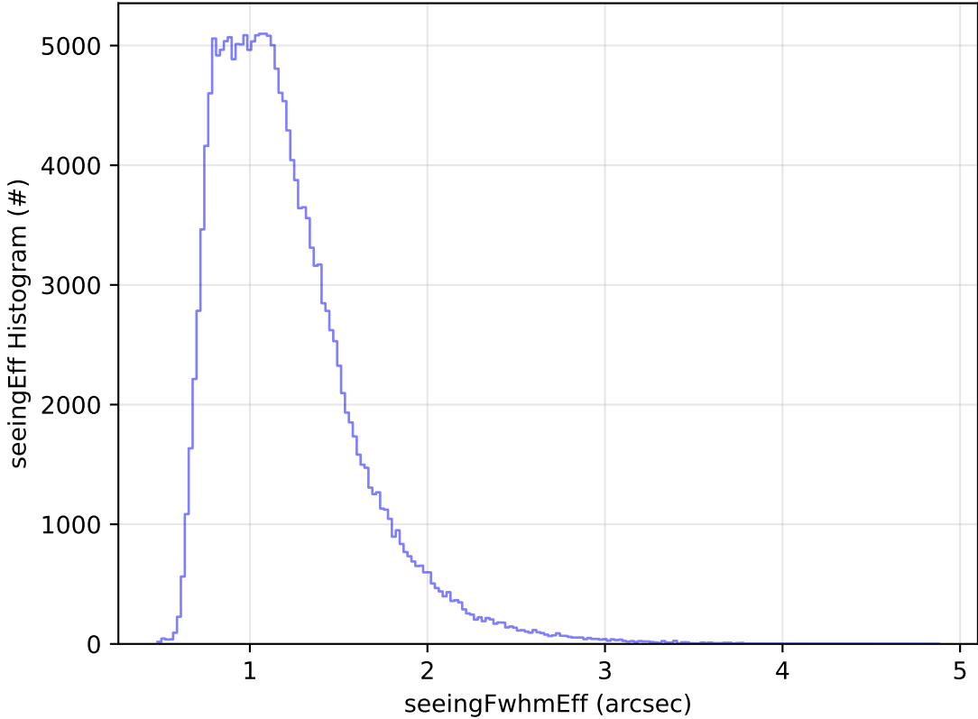
too_combined_no_nss_s10.0_v3.4_10yrs WFD g band: seeingEff Histogram
