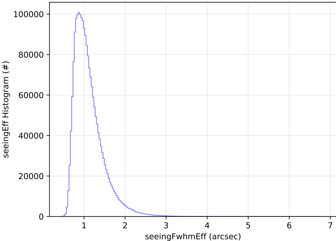
too_combined_no_nss_s10.0_v3.4_10yrs WFD all bands: seeingEff Histogram
