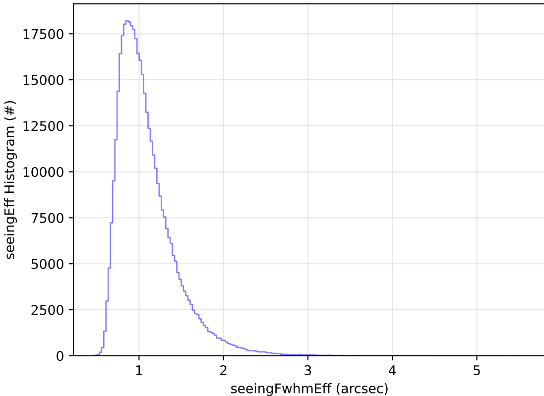
too_combined_no_nss_s10.0_v3.4_10yrs All sky z band: seeingEff Histogram
