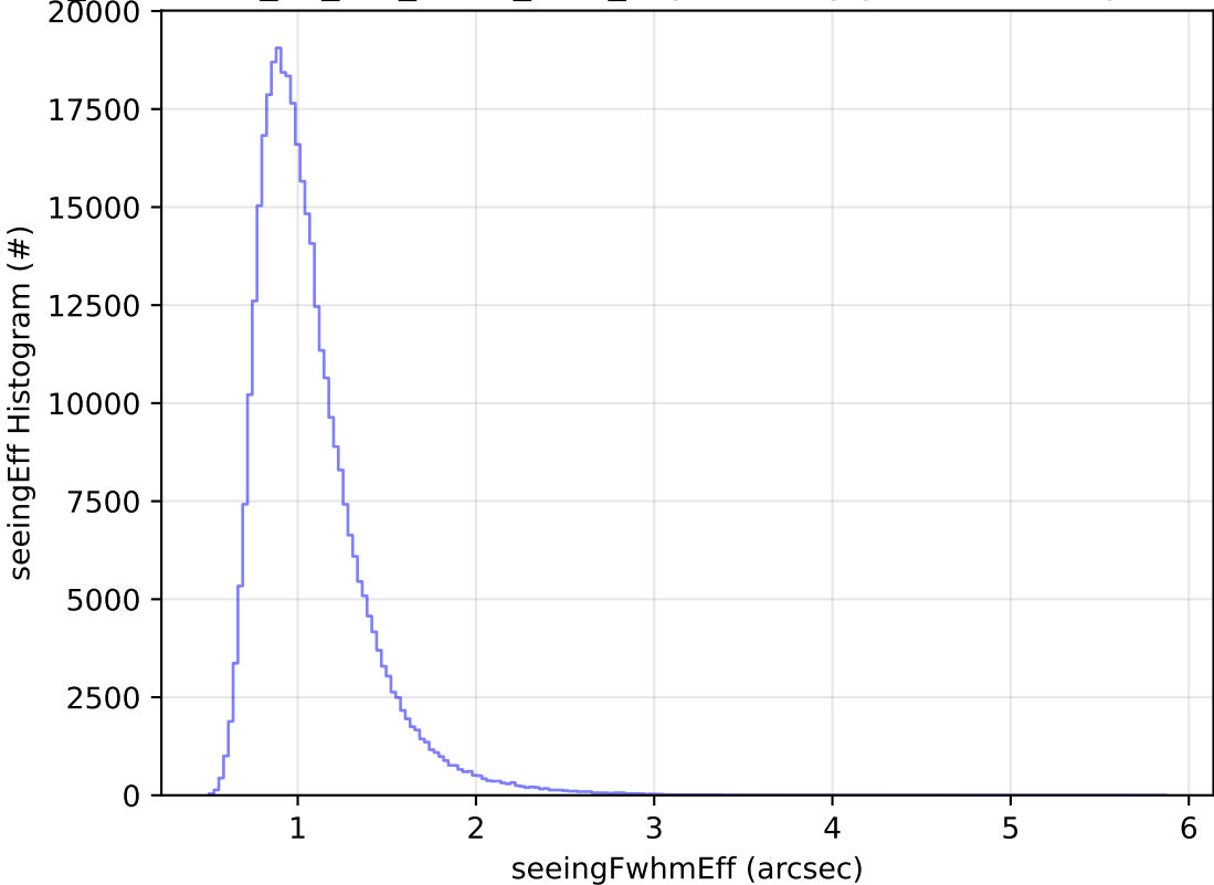
too_combined_no_nss_s10.0_v3.4_10yrs All sky y band: seeingEff Histogram
