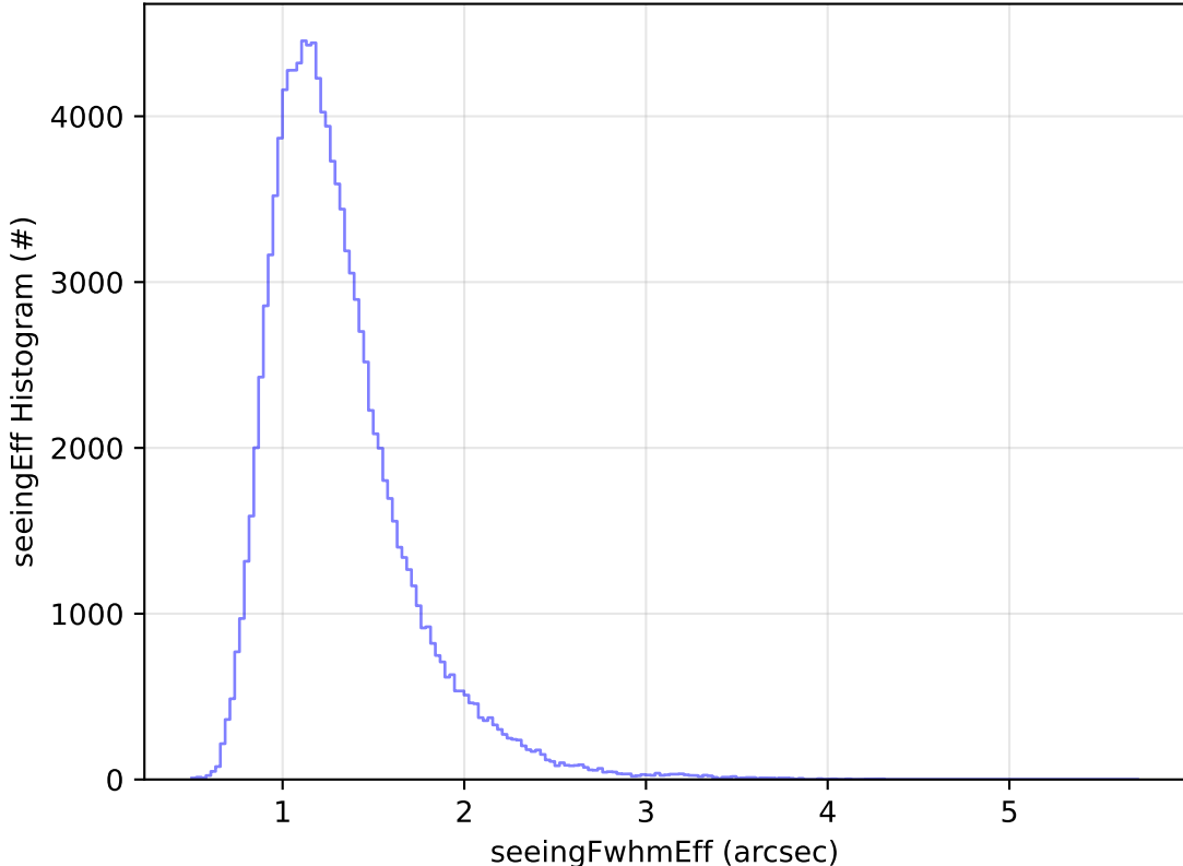
too_combined_no_nss_s10.0_v3.4_10yrs All sky u band: seeingEff Histogram
