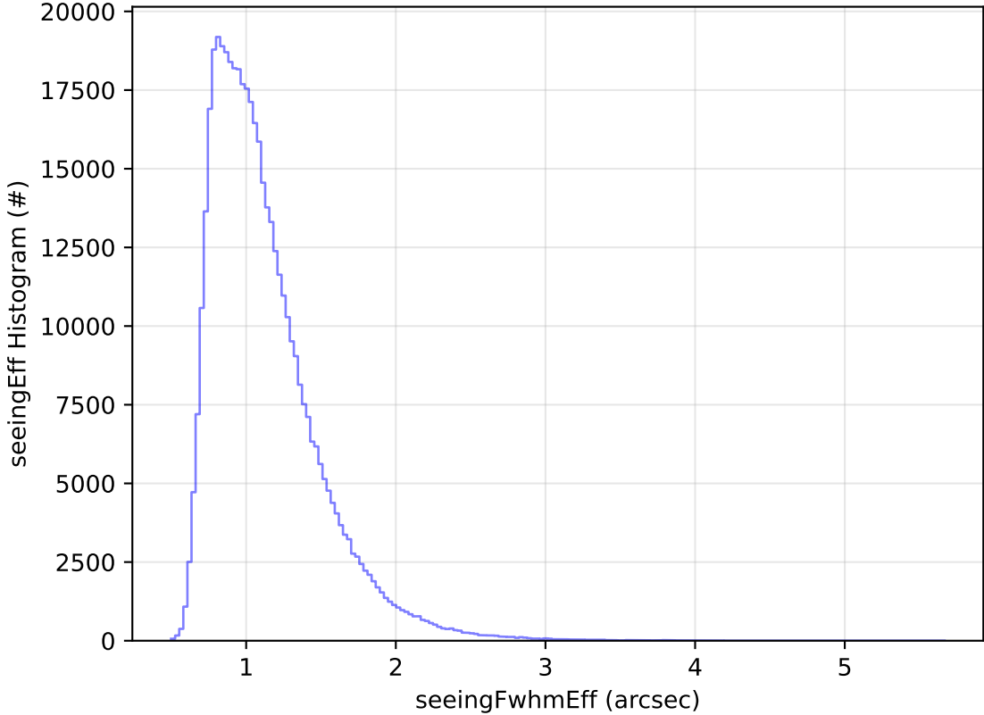
too_combined_no_nss_s10.0_v3.4_10yrs All sky r band: seeingEff Histogram
