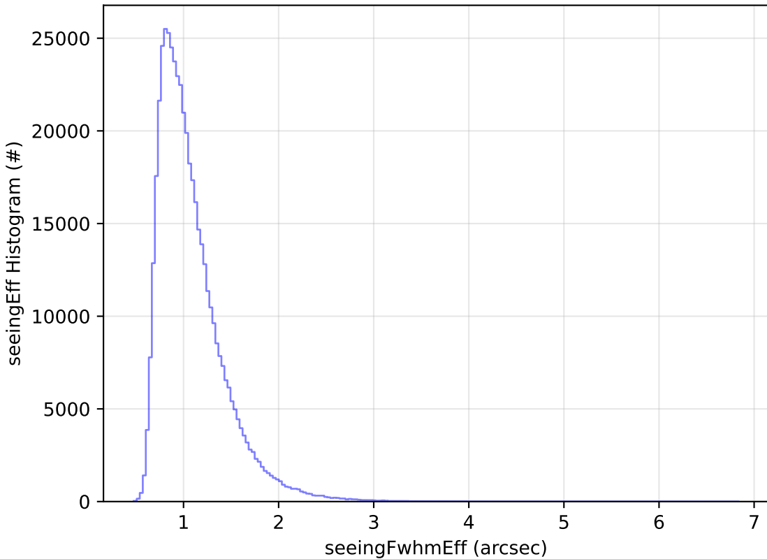
too_combined_no_nss_s10.0_v3.4_10yrs All sky i band: seeingEff Histogram
