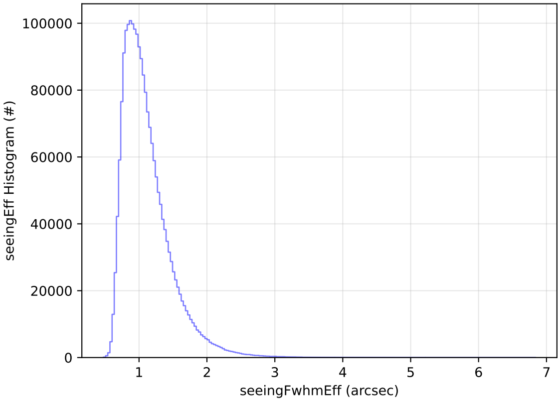
too_combined_no_nss_s10.0_v3.4_10yrs All sky all bands: seeingEff Histogram
