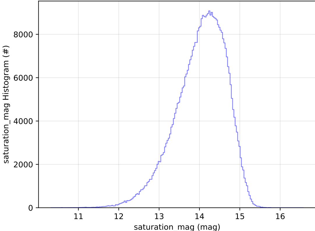
too_combined_no_nss_s10.0_v3.4_10yrs WFD z band: saturation_mag Histogram
