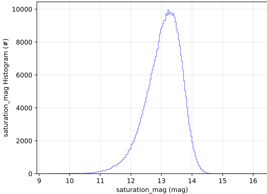
too_combined_no_nss_s10.0_v3.4_10yrs WFD y band: saturation_mag Histogram
