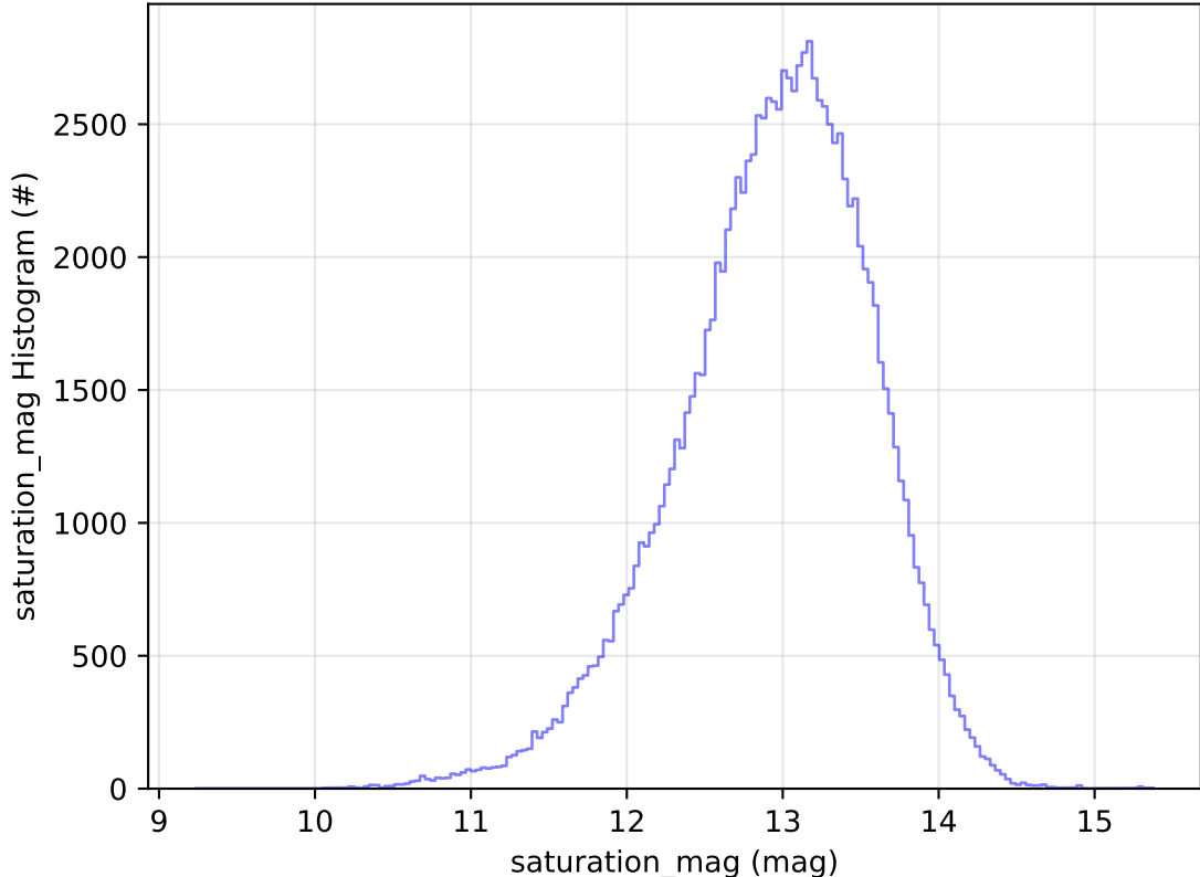
too_combined_no_nss_s10.0_v3.4_10yrs WFD u band: saturation_mag Histogram
