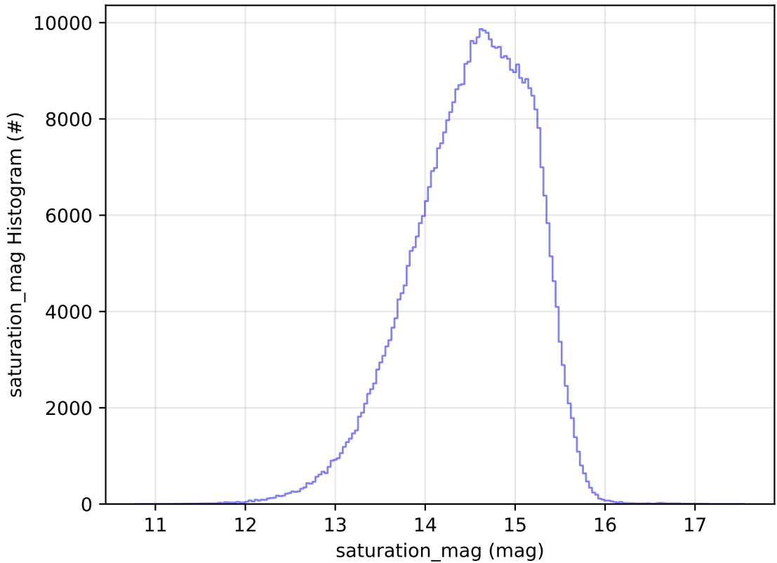
too_combined_no_nss_s10.0_v3.4_10yrs WFD r band: saturation_mag Histogram
