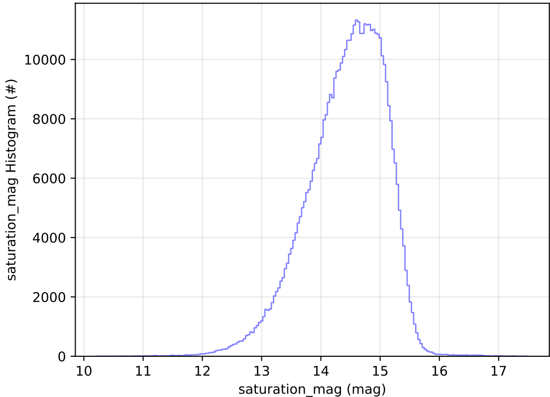
too_combined_no_nss_s10.0_v3.4_10yrs WFD i band: saturation_mag Histogram
