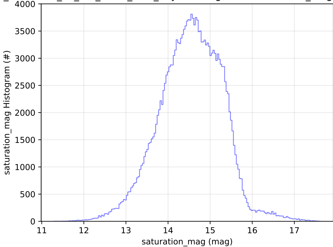
too_combined_no_nss_s10.0_v3.4_10yrs WFD g band: saturation_mag Histogram
