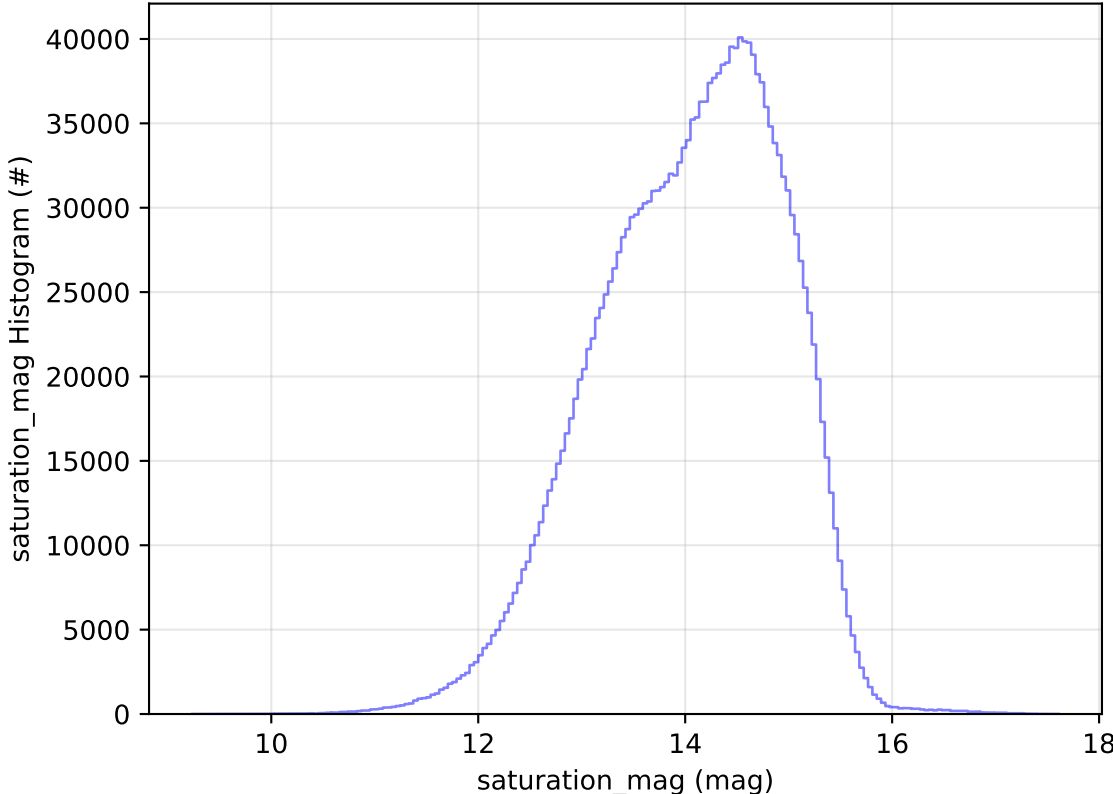
too_combined_no_nss_s10.0_v3.4_10yrs WFD all bands: saturation_mag Histogram
