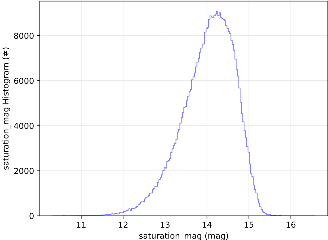
too_combined_no_nss_s10.0_v3.4_10yrs All sky z band: saturation_mag Histogram
