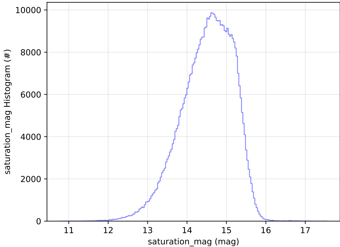
too_combined_no_nss_s10.0_v3.4_10yrs All sky r band: saturation_mag Histogram
