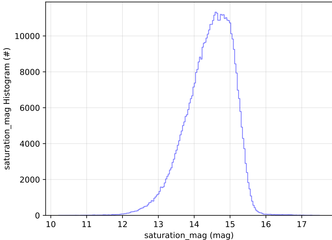
too_combined_no_nss_s10.0_v3.4_10yrs All sky i band: saturation_mag Histogram
