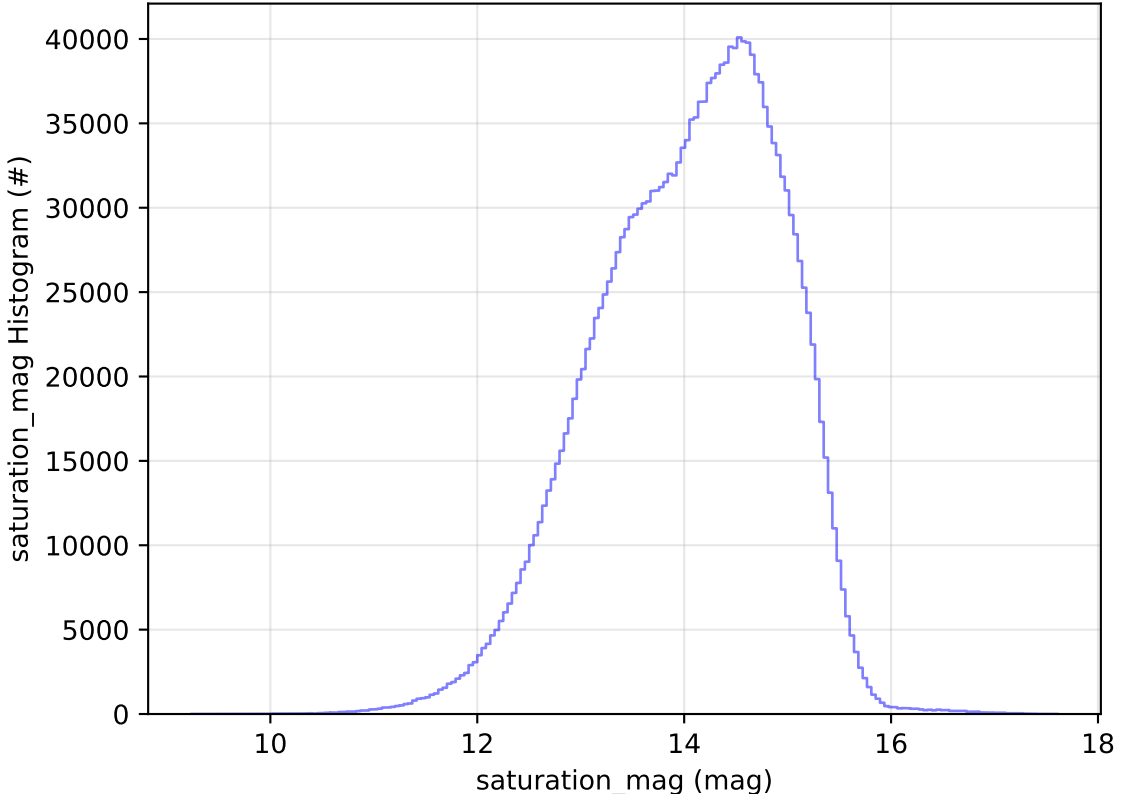
too_combined_no_nss_s10.0_v3.4_10yrs All sky all bands: saturation_mag Histogram
