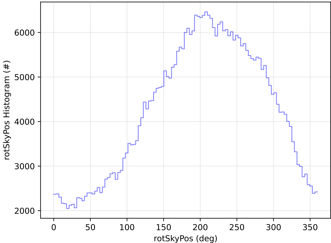
too_combined_no_nss_s10.0_v3.4_10yrs WFD z band: rotSkyPos Histogram
