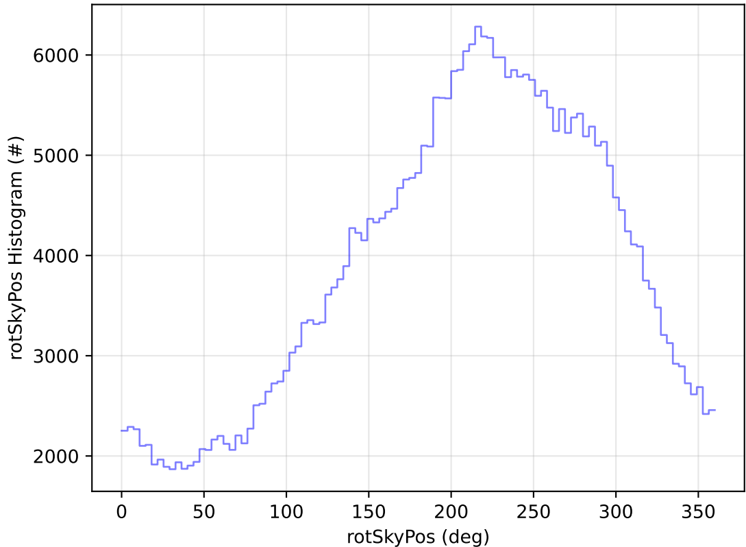
too_combined_no_nss_s10.0_v3.4_10yrs WFD y band: rotSkyPos Histogram
