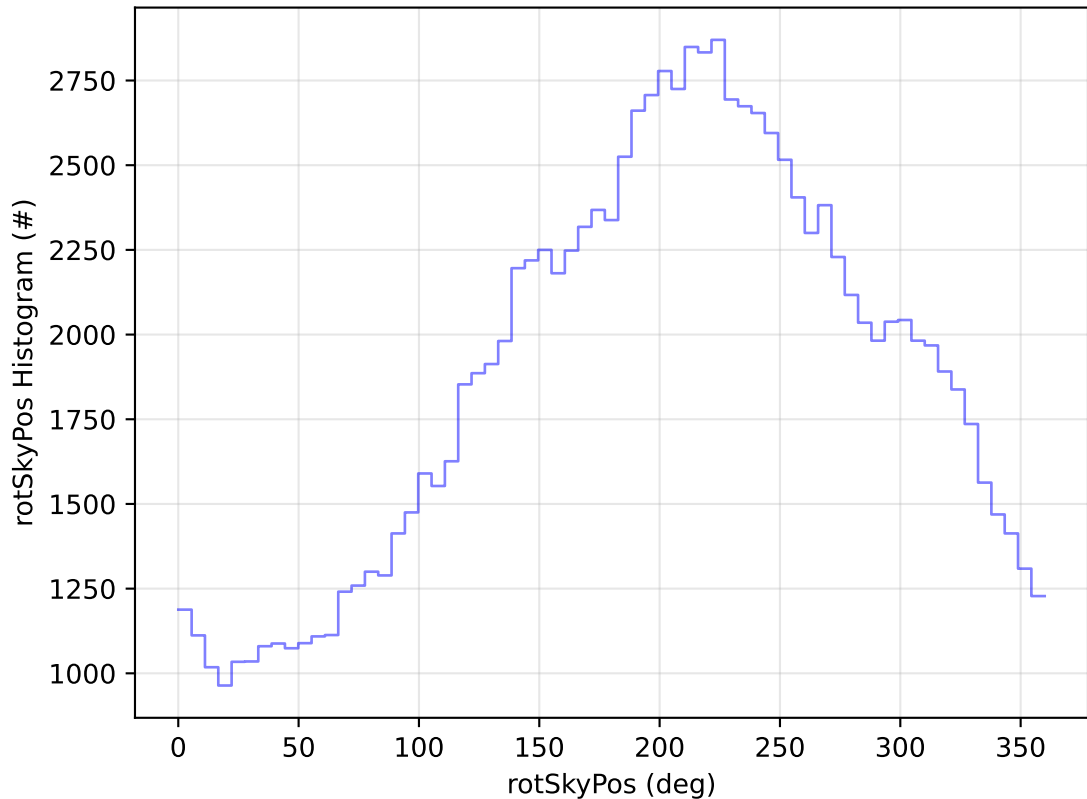
too_combined_no_nss_s10.0_v3.4_10yrs WFD u band: rotSkyPos Histogram
