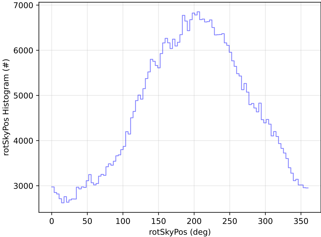
too_combined_no_nss_s10.0_v3.4_10yrs WFD r band: rotSkyPos Histogram
