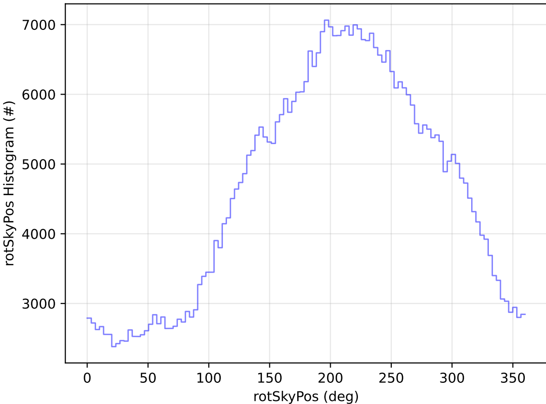
too_combined_no_nss_s10.0_v3.4_10yrs WFD i band: rotSkyPos Histogram
