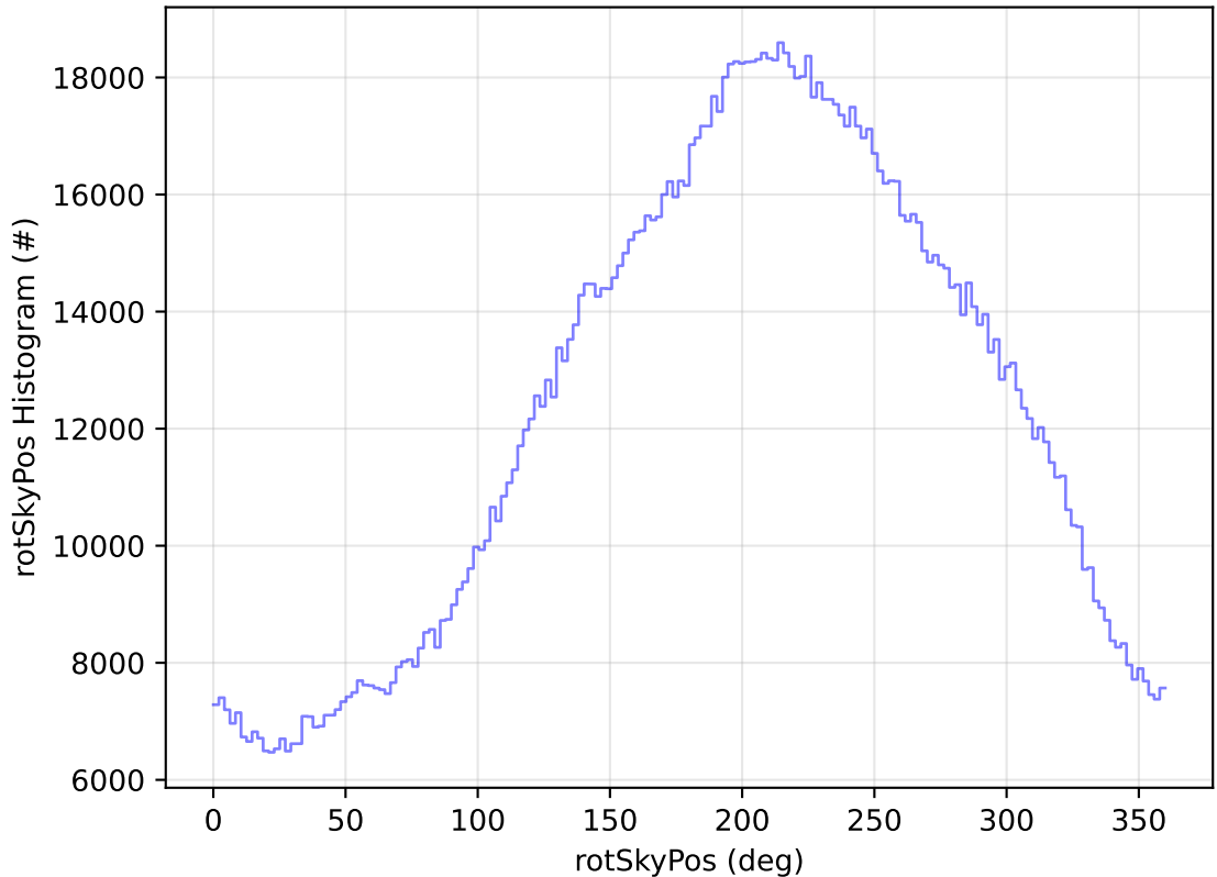
too_combined_no_nss_s10.0_v3.4_10yrs WFD all bands: rotSkyPos Histogram
