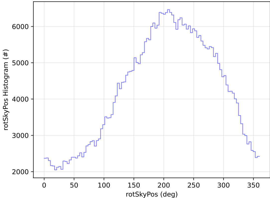
too_combined_no_nss_s10.0_v3.4_10yrs All sky z band: rotSkyPos Histogram
