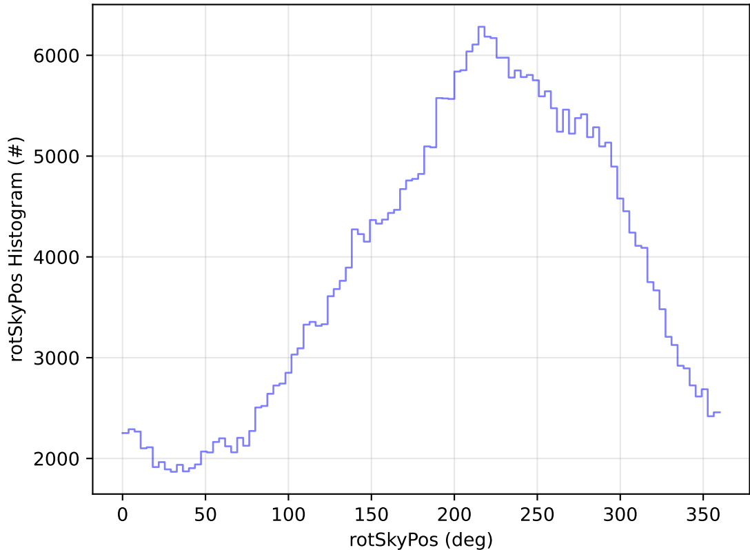
too_combined_no_nss_s10.0_v3.4_10yrs All sky y band: rotSkyPos Histogram
