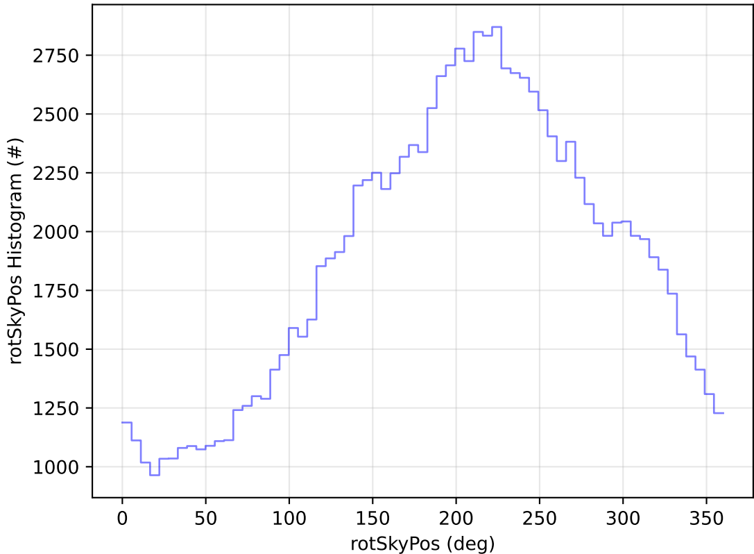
too_combined_no_nss_s10.0_v3.4_10yrs All sky u band: rotSkyPos Histogram
