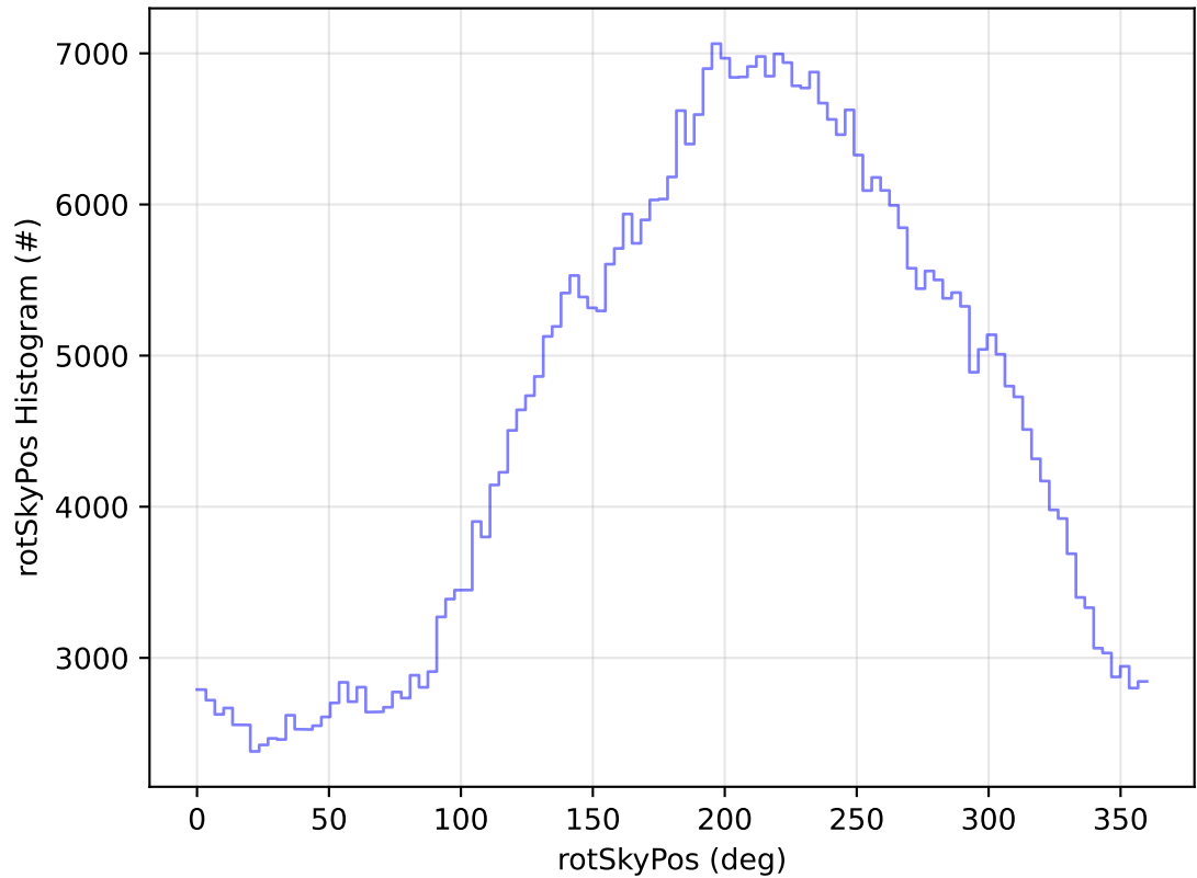
too_combined_no_nss_s10.0_v3.4_10yrs All sky i band: rotSkyPos Histogram
