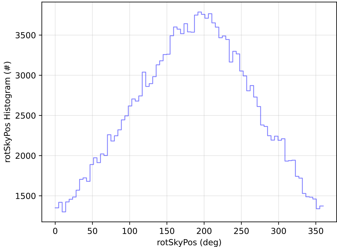
too_combined_no_nss_s10.0_v3.4_10yrs All sky g band: rotSkyPos Histogram
