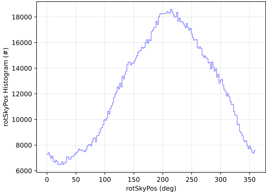
too_combined_no_nss_s10.0_v3.4_10yrs All sky all bands: rotSkyPos Histogram
