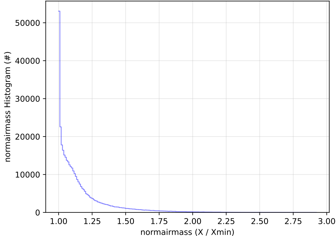
too_combined_no_nss_s10.0_v3.4_10yrs WFD y band: normairmass Histogram
