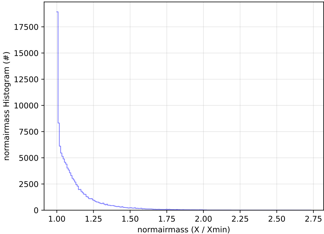
too_combined_no_nss_s10.0_v3.4_10yrs WFD u band: normairmass Histogram
