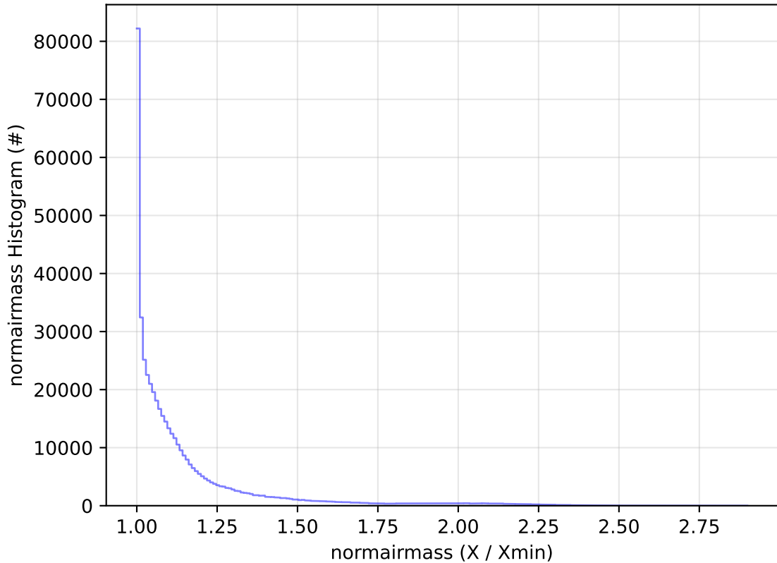
too_combined_no_nss_s10.0_v3.4_10yrs WFD r band: normairmass Histogram
