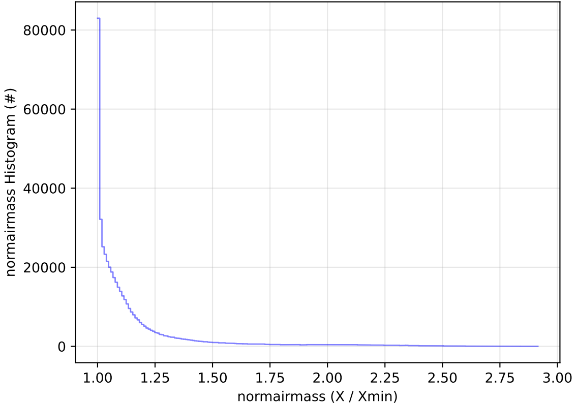
too_combined_no_nss_s10.0_v3.4_10yrs WFD i band: normairmass Histogram
