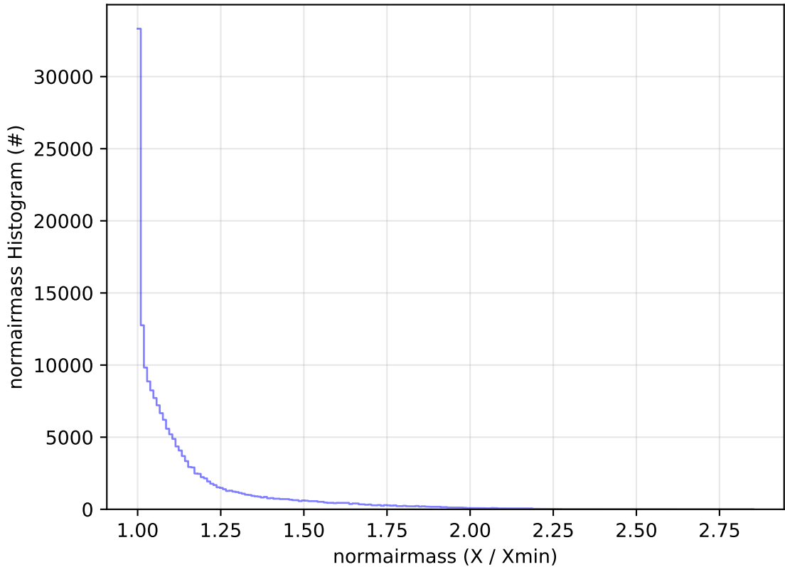
too_combined_no_nss_s10.0_v3.4_10yrs WFD g band: normairmass Histogram
