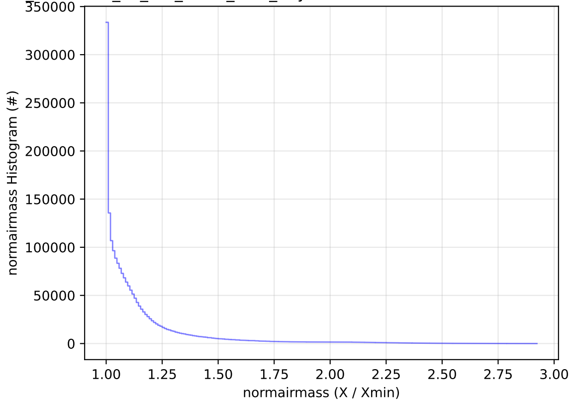
too_combined_no_nss_s10.0_v3.4_10yrs WFD all bands: normairmass Histogram
