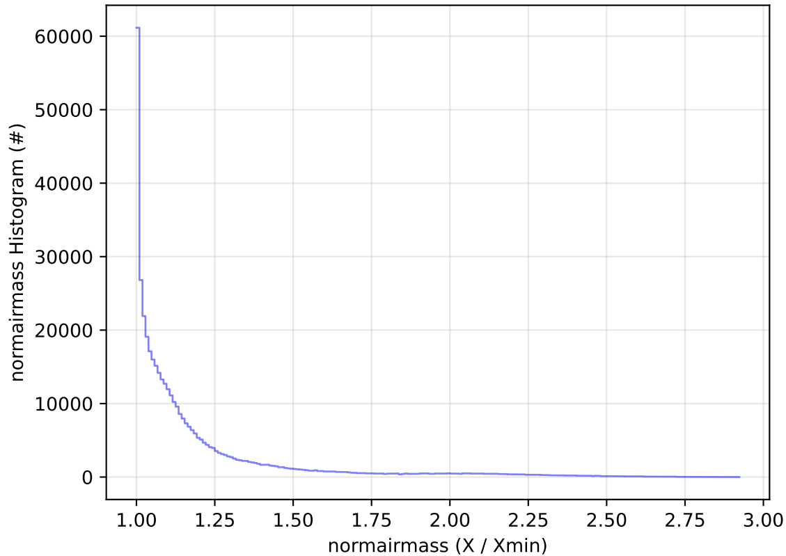
too_combined_no_nss_s10.0_v3.4_10yrs All sky z band: normairmass Histogram
