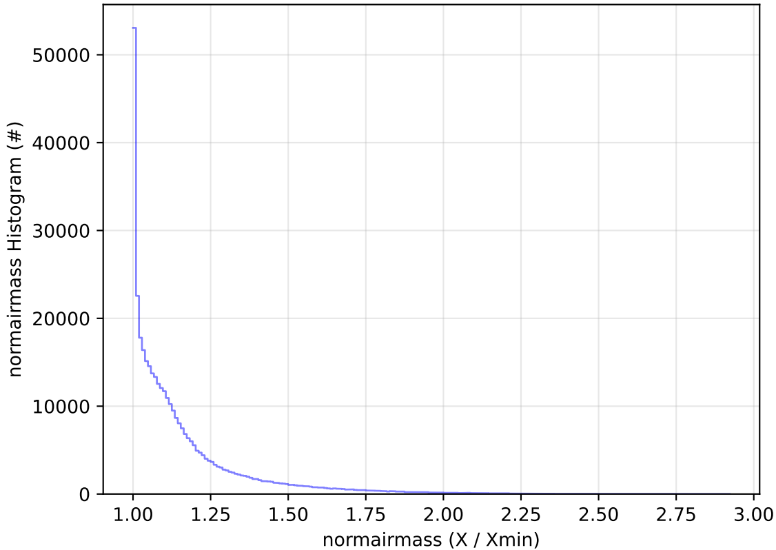
too_combined_no_nss_s10.0_v3.4_10yrs All sky y band: normairmass Histogram
