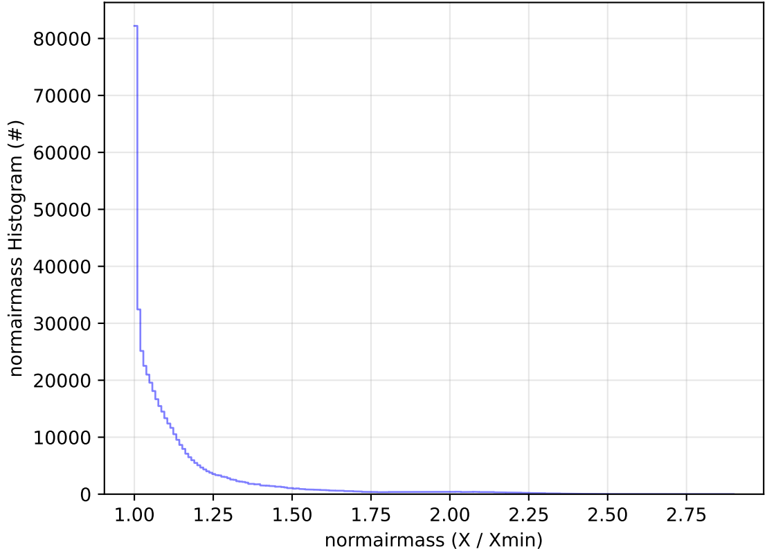
too_combined_no_nss_s10.0_v3.4_10yrs All sky r band: normairmass Histogram
