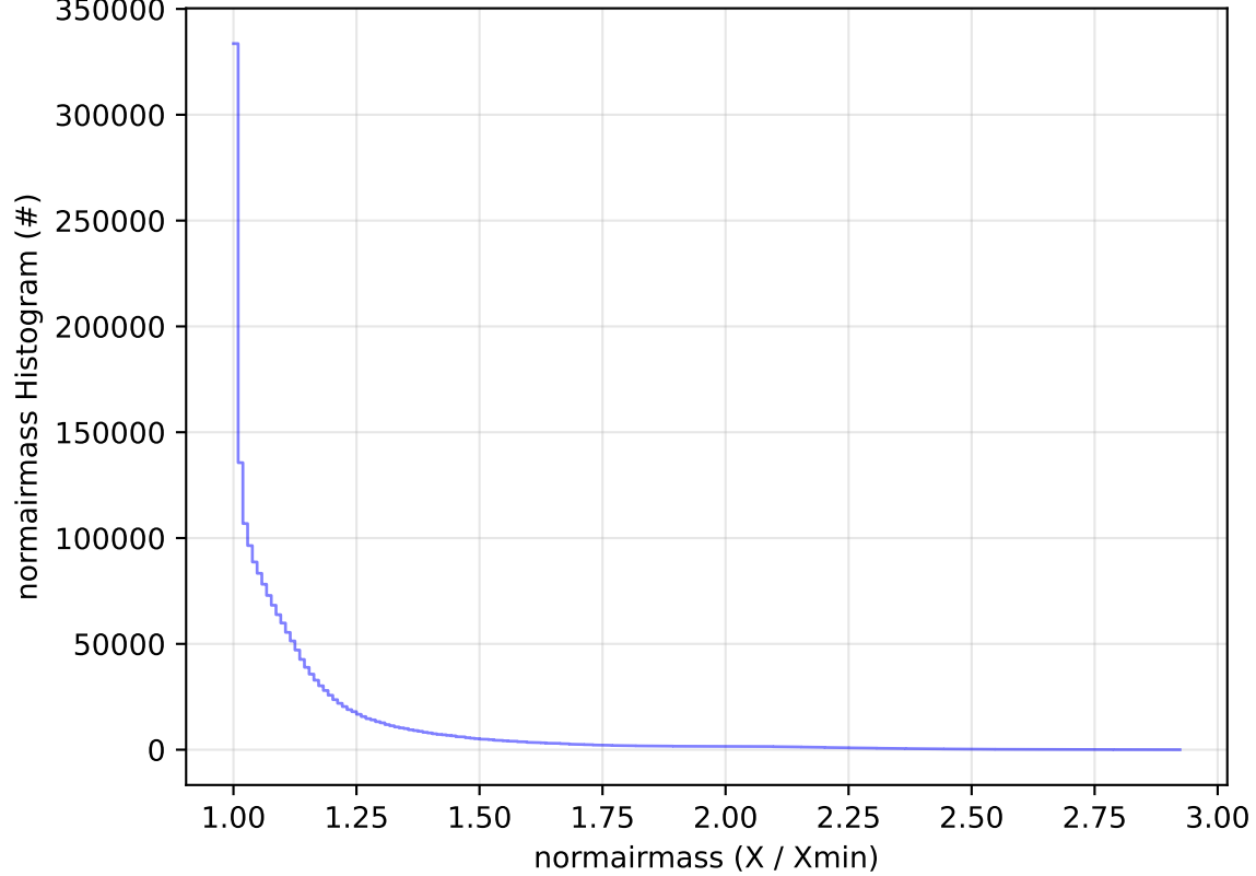
too_combined_no_nss_s10.0_v3.4_10yrs All sky all bands: normairmass Histogram
