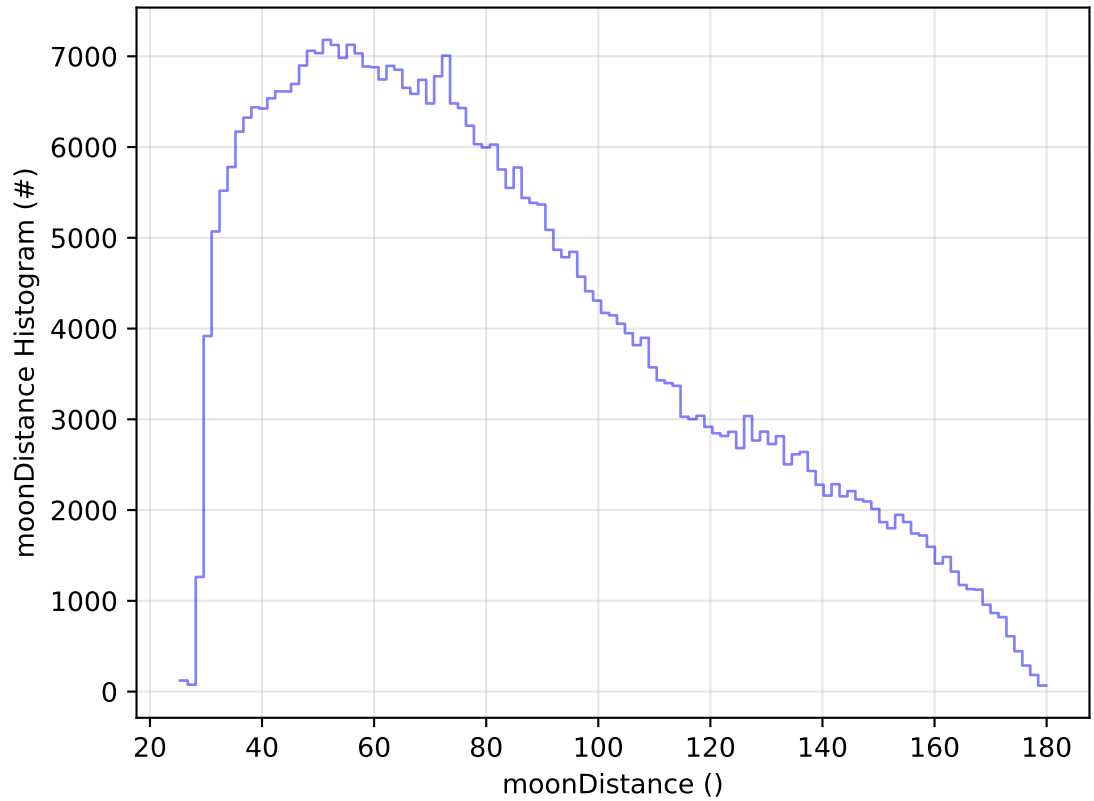
too_combined_no_nss_s10.0_v3.4_10yrs WFD z band: moonDistance Histogram
