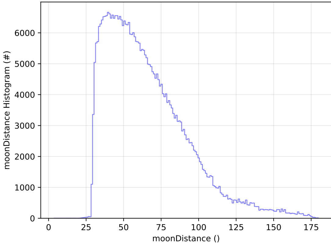
too_combined_no_nss_s10.0_v3.4_10yrs WFD y band: moonDistance Histogram
