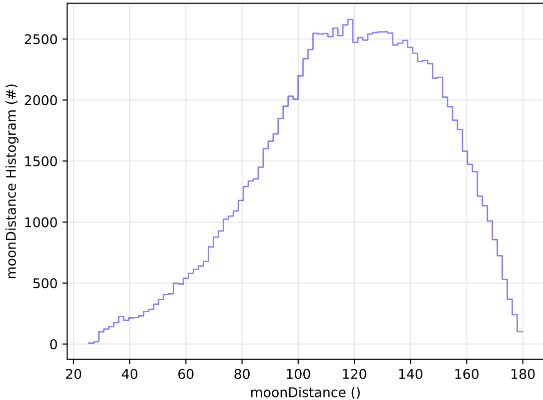
too_combined_no_nss_s10.0_v3.4_10yrs WFD u band: moonDistance Histogram
