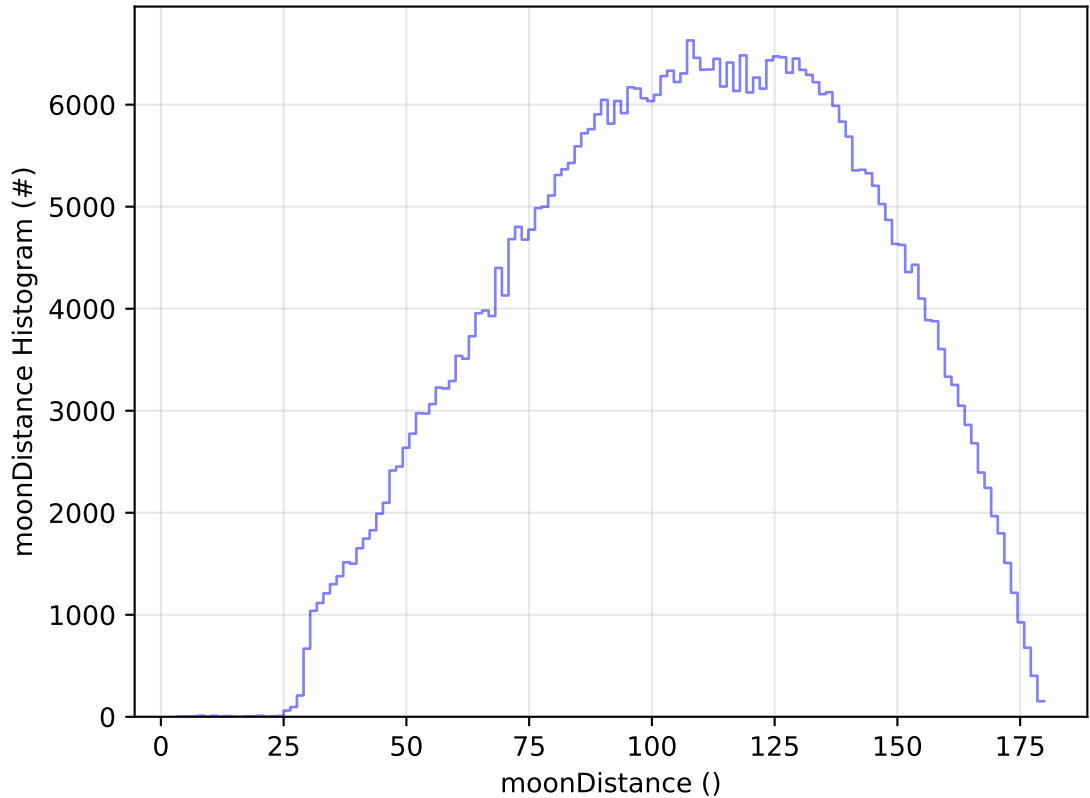
too_combined_no_nss_s10.0_v3.4_10yrs WFD r band: moonDistance Histogram
