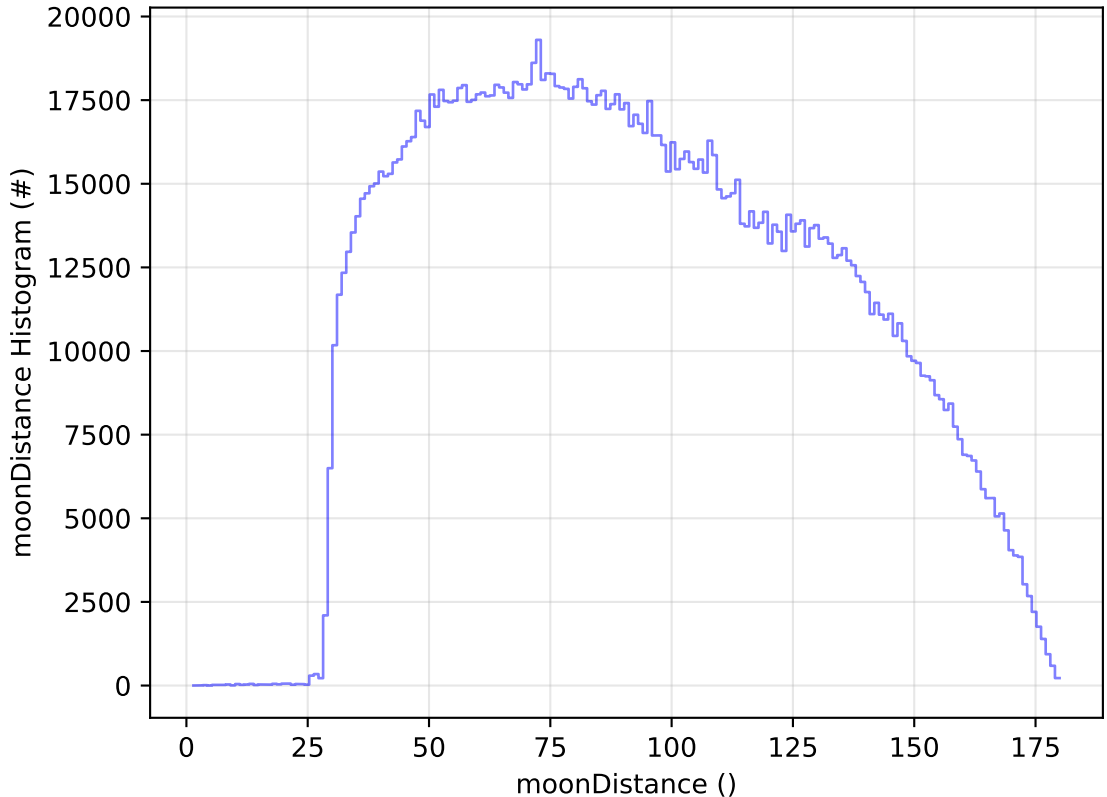
too_combined_no_nss_s10.0_v3.4_10yrs WFD all bands: moonDistance Histogram
