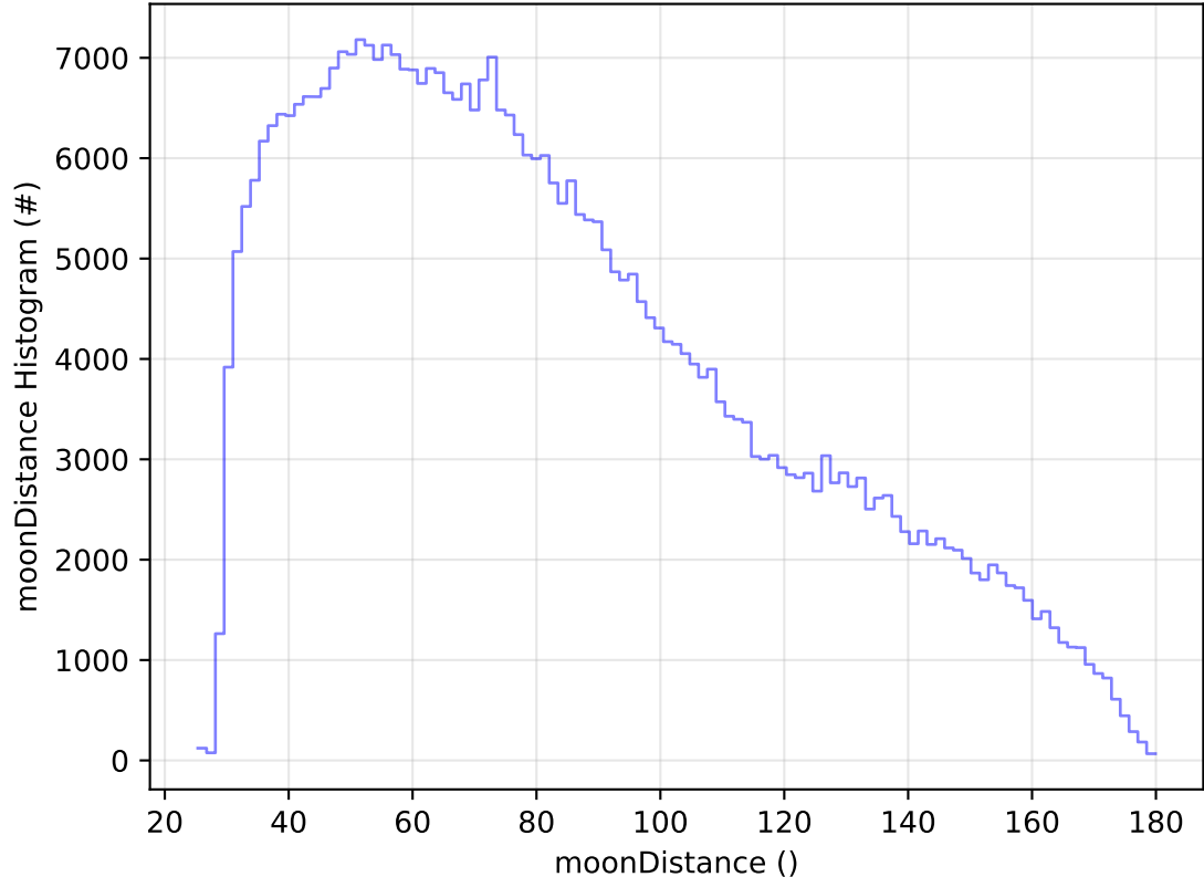
too_combined_no_nss_s10.0_v3.4_10yrs All sky z band: moonDistance Histogram
