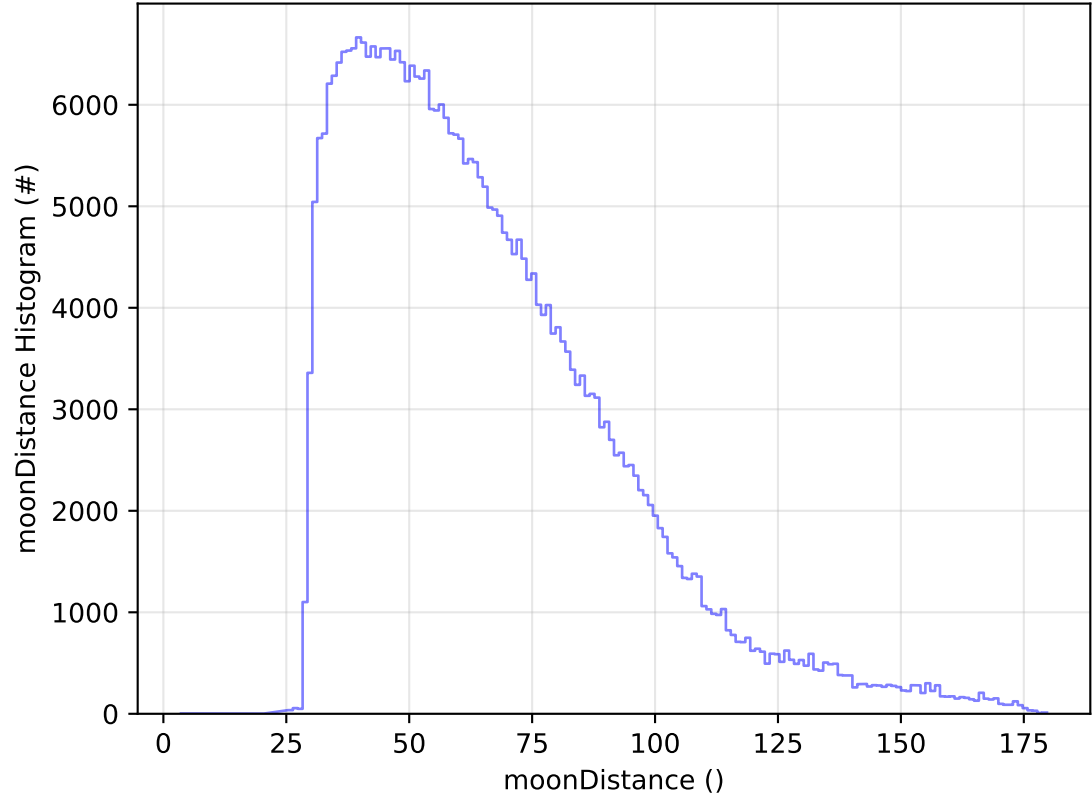
too_combined_no_nss_s10.0_v3.4_10yrs All sky y band: moonDistance Histogram
