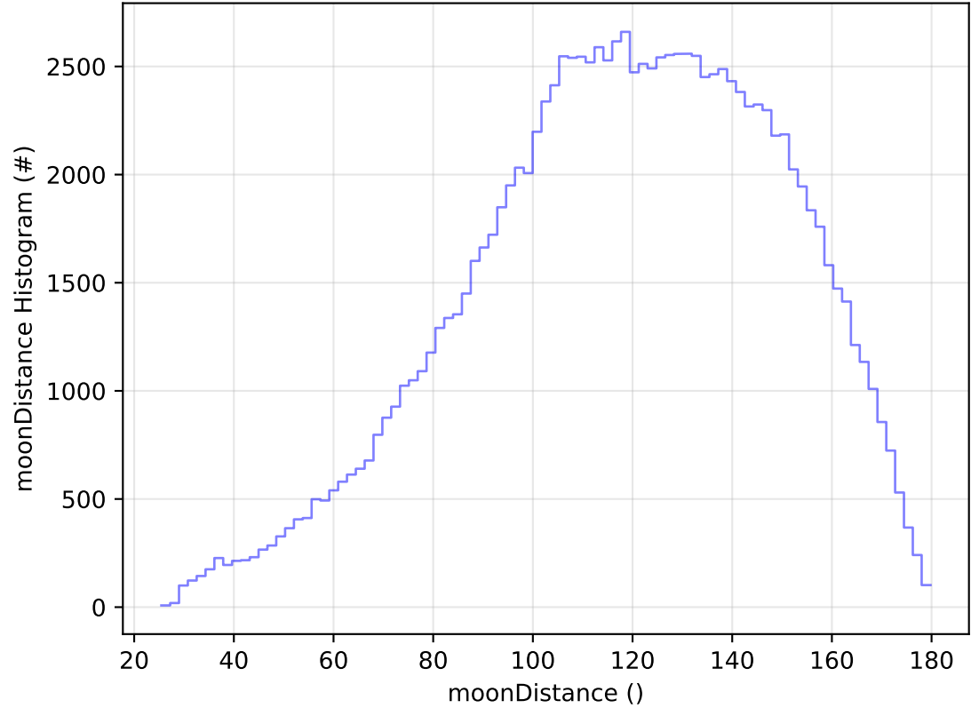
too_combined_no_nss_s10.0_v3.4_10yrs All sky u band: moonDistance Histogram
